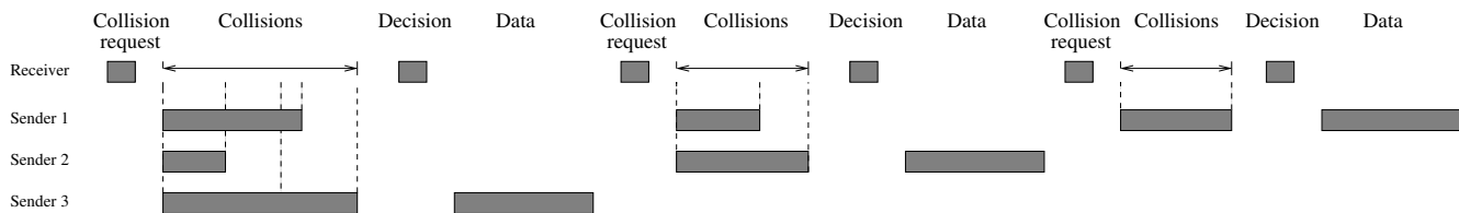
Figure 3: Strawman senders “draw straws” to gain channel access by simultaneously transmitting COLLISION packets with randomly picked lengths, resulting in a deliberate collision. The receiver does not have to correctly decode any of the COLLISION packets, but only needs to measure the duration of the collision. The sender with the longest COLLISION gains channel access and sends its packet. The process is repeated until all packets are sent.
